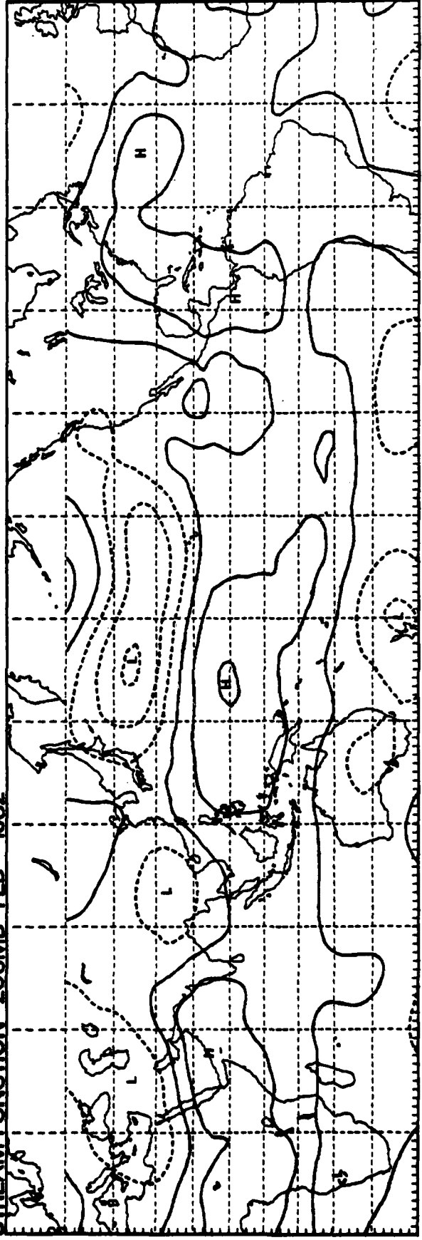
STREAM FUNCTION 200MB FEB 1982
